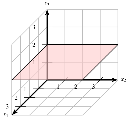
Abb. 5: E_7 : x_3 = 2
