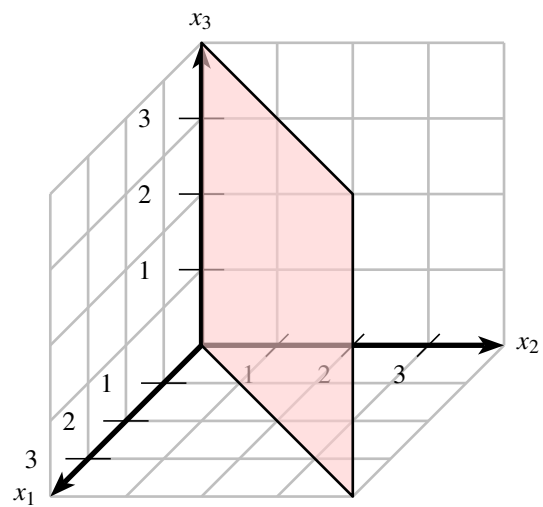
Abb. 6: E_8 : x_1 = x_2
