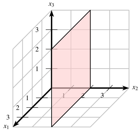
Abb. 4: E_6 : x_2 = 2
