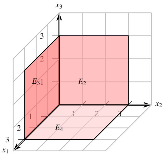
Abb. 2: E_2 : x_1 = 0; E_3 : x_2 = 0; E_4 : x_3 = 0
