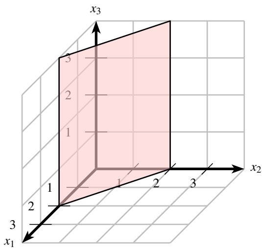
Abb. 3: E_5 : x_1 + x_2 = 2
